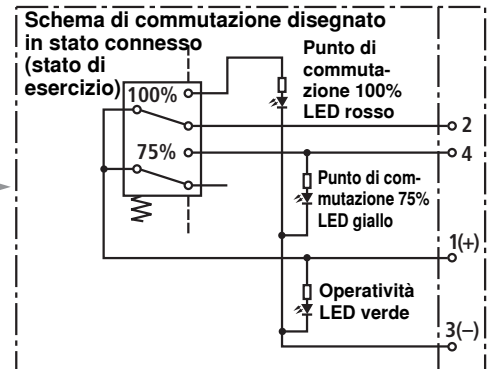
ABZFBV-E2SP-M12X1-1X/-DIN
