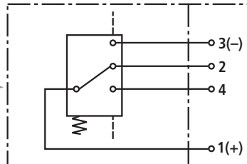
ABZFFV-E1SP-M12X1-1X/-DIN
